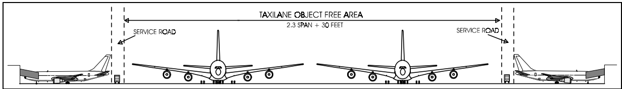
FIGURE 13. NLA ON DUAL TAXILANE
