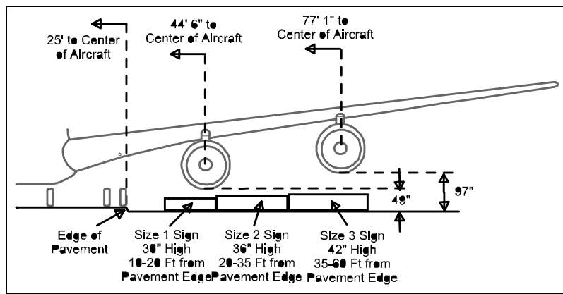
FIGURE 15. NLA SIGN CLEARANCE
