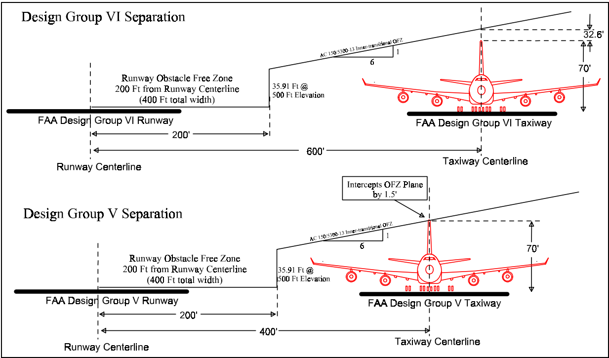
FIGURE 11. DEPICTION OF NLA ON DESIGN GROUP V AND VI PARALLEL TAXIWAY
