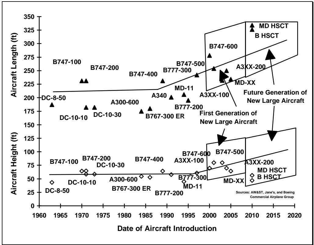
FIGURE 4. AIRCRAFT LENGTH AND HEIGHT TRENDS
