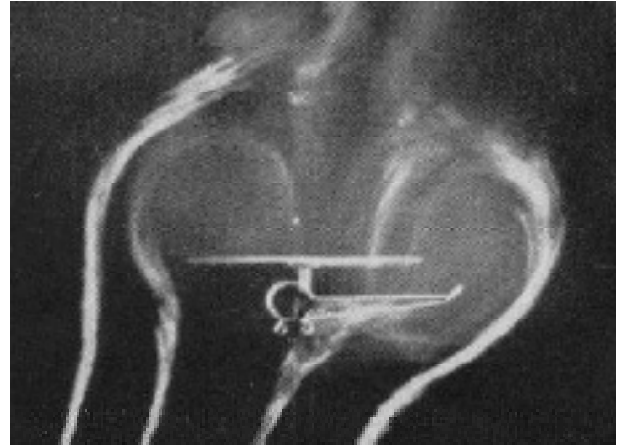
Figure 1. Smoke flow visualization of a rotor in vortex ring state (Drees, Ref. 20).
