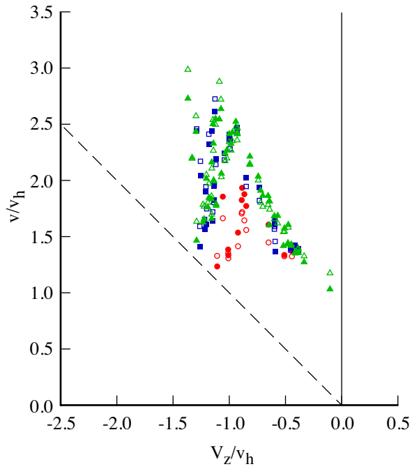
Figure 23b. Betzina (2001) wind tunnel test: influence of image plane; \sigma = 0.1194 , \theta_{tw} = -41 deg; nonaxial flow, \alpha = 60 deg.
