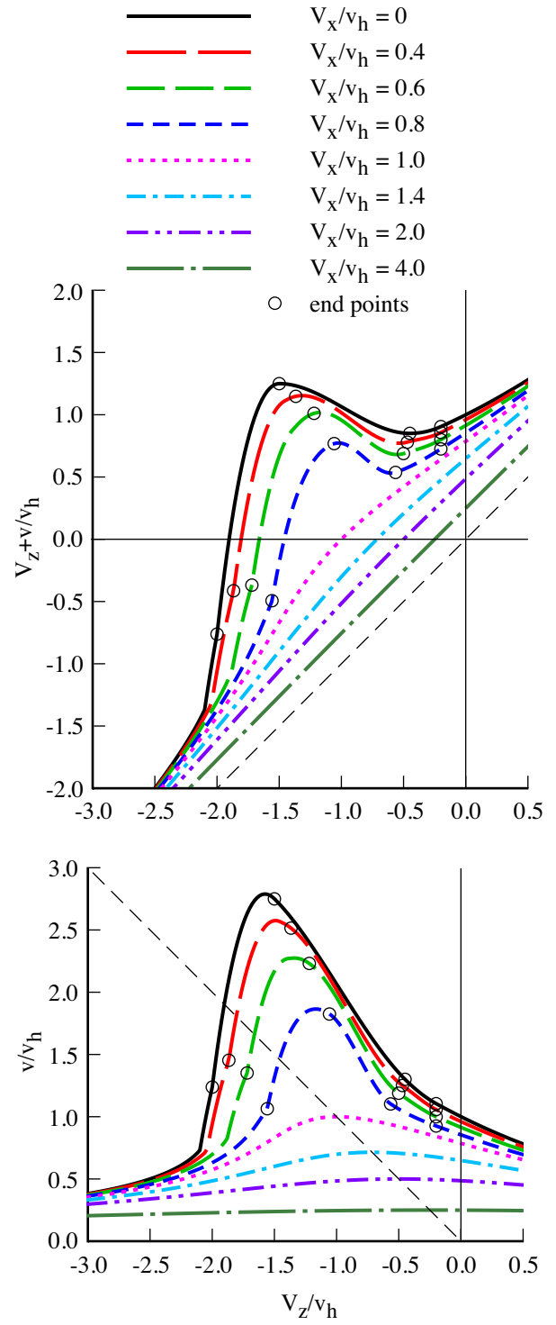
Figure 39. VRS model.
