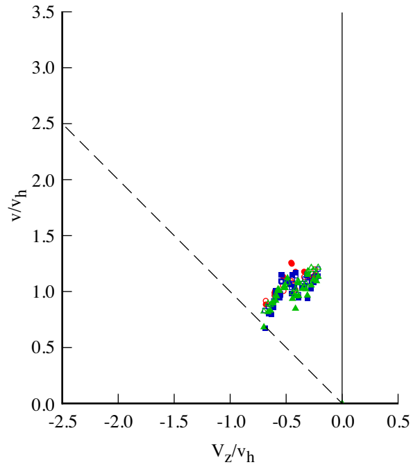
Figure 23c. Betzina (2001) wind tunnel test: influence of image plane; \sigma = 0.1194 , \theta_{tw} = -41 deg; nonaxial flow, \alpha = 30 deg.
