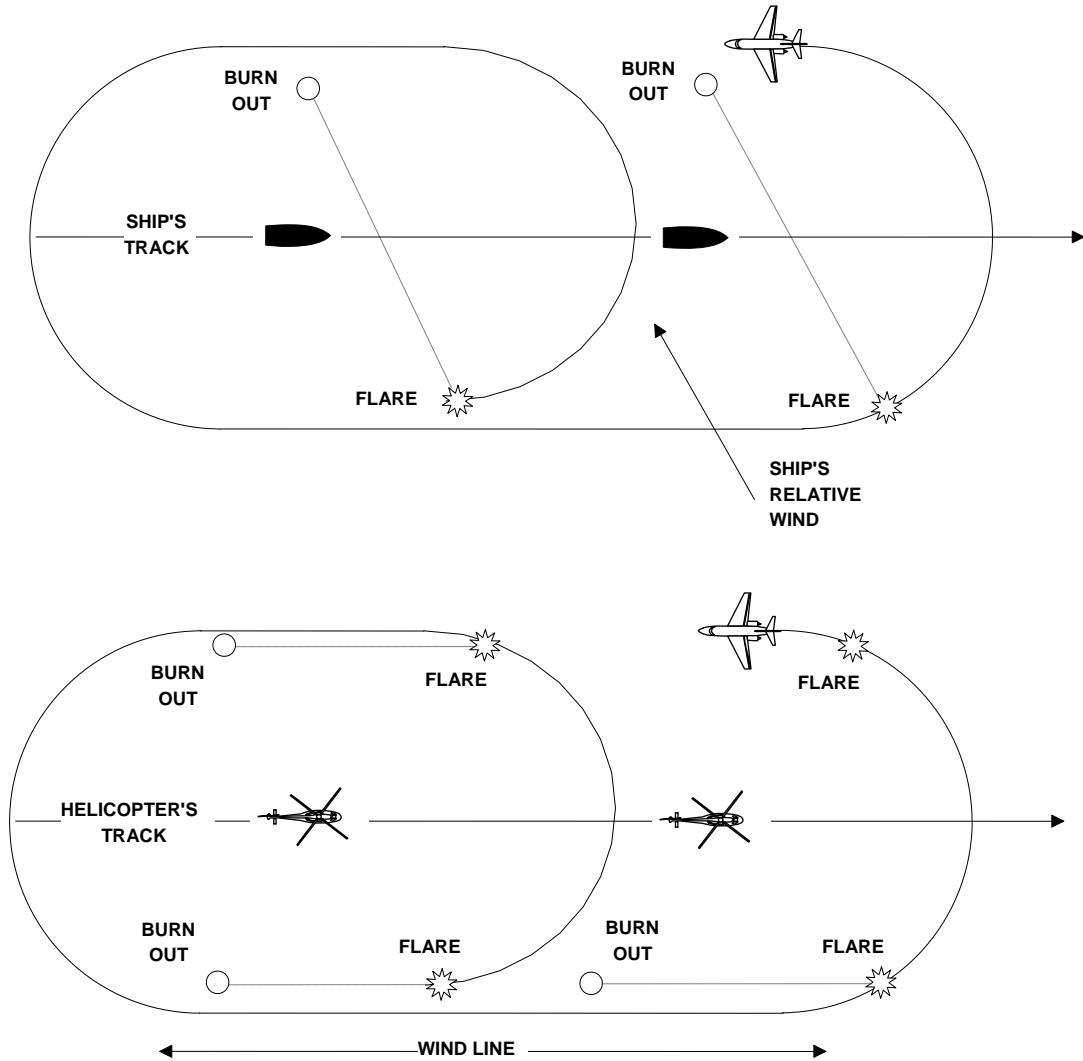
Figure H-46 Flare Single-Unit (FS)
