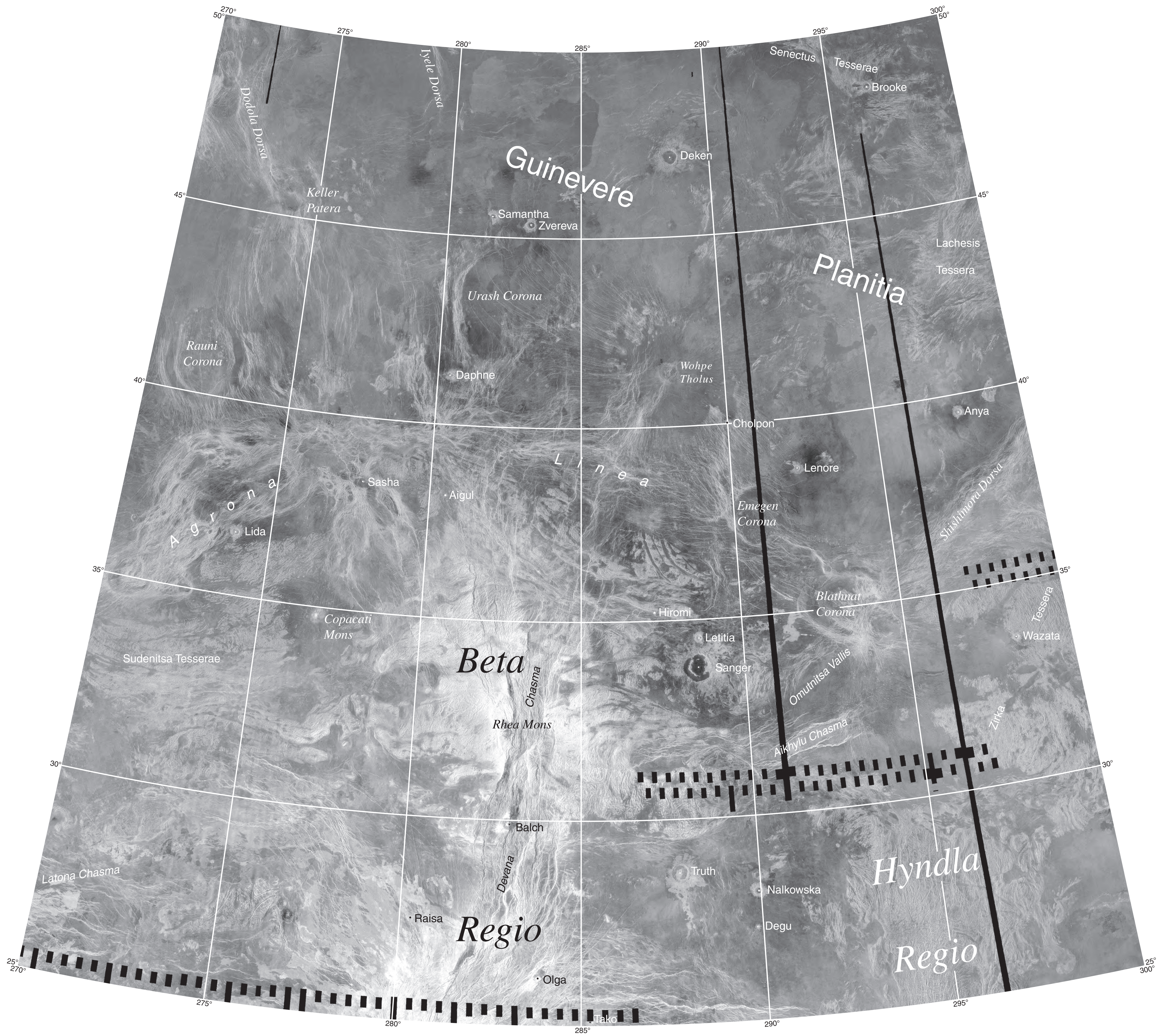
Beta Regio, V-17 Lambert projection
