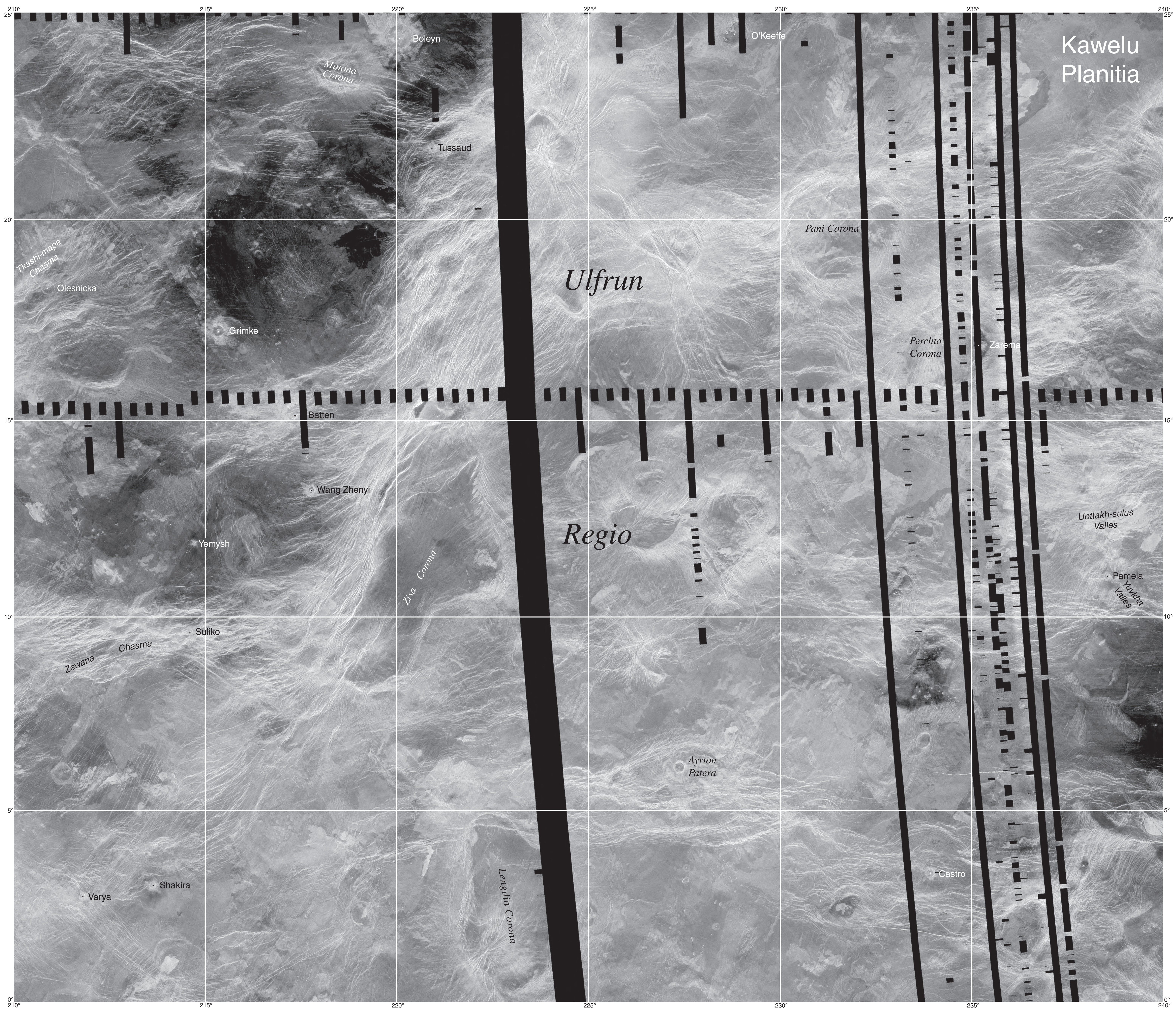
Ulfrun Regio, V-27 Mercator projection
