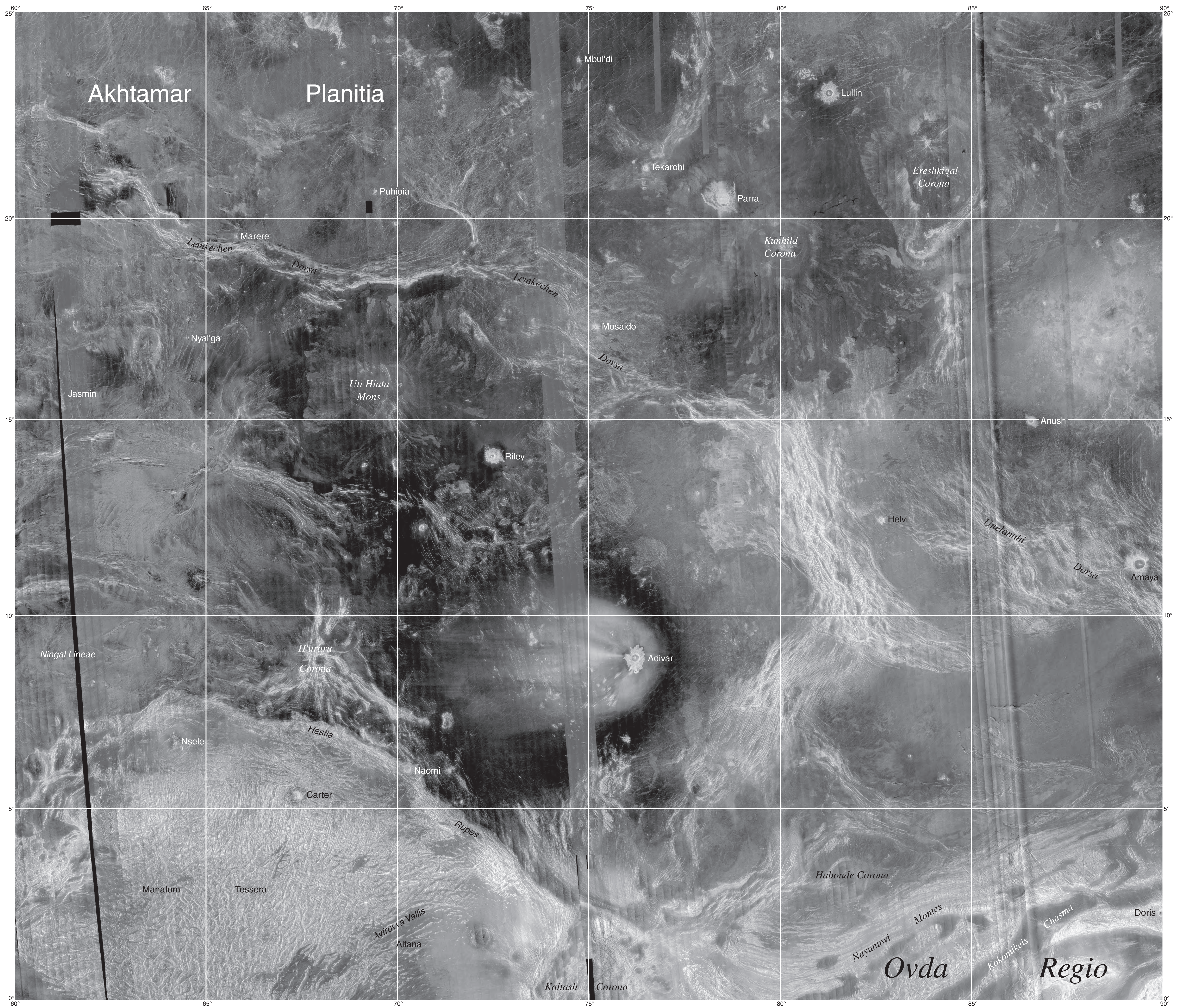
Hestia Rupes, V-22 Mercator projection
