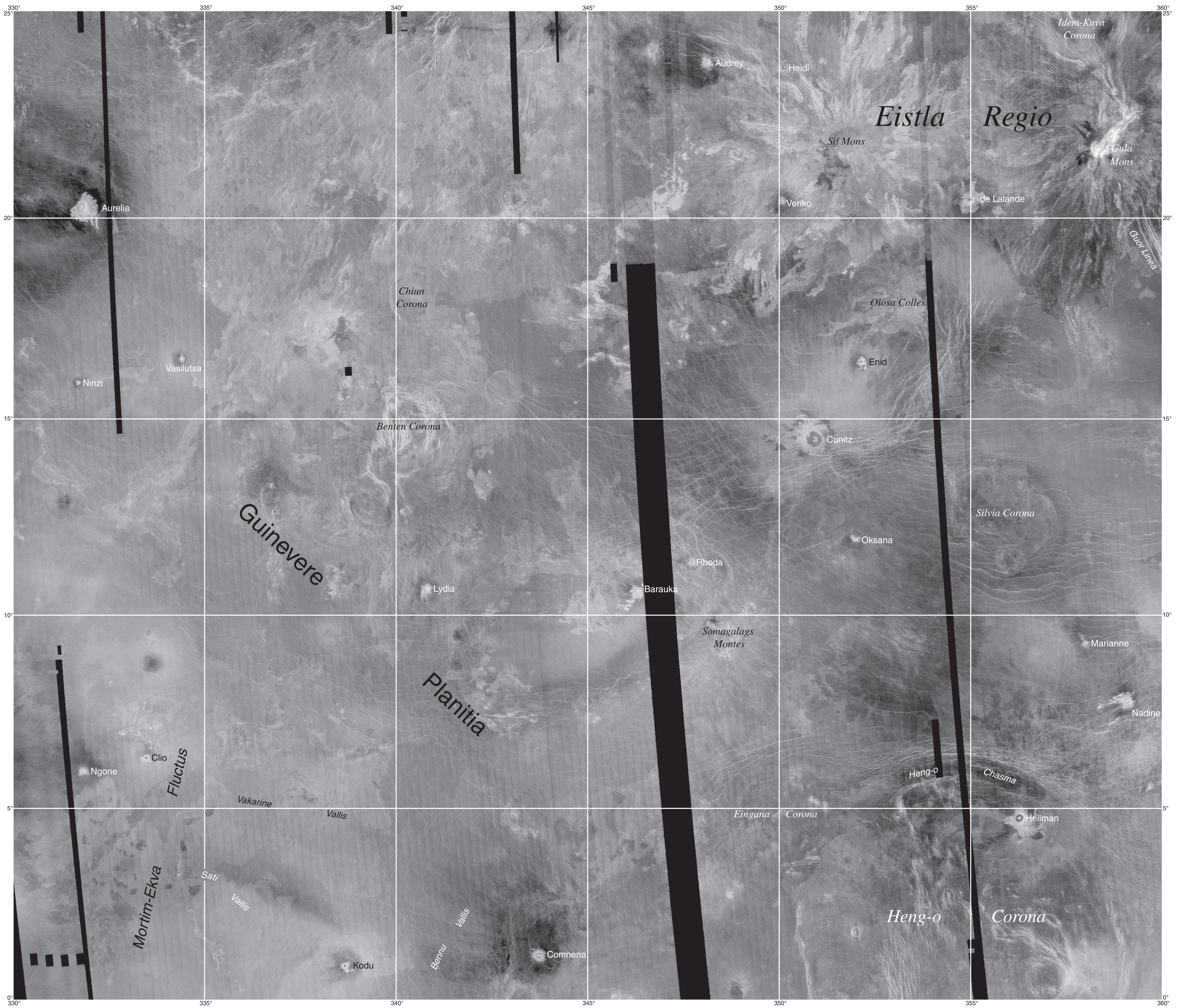
Sif Mons, V-31 Mercator projection
