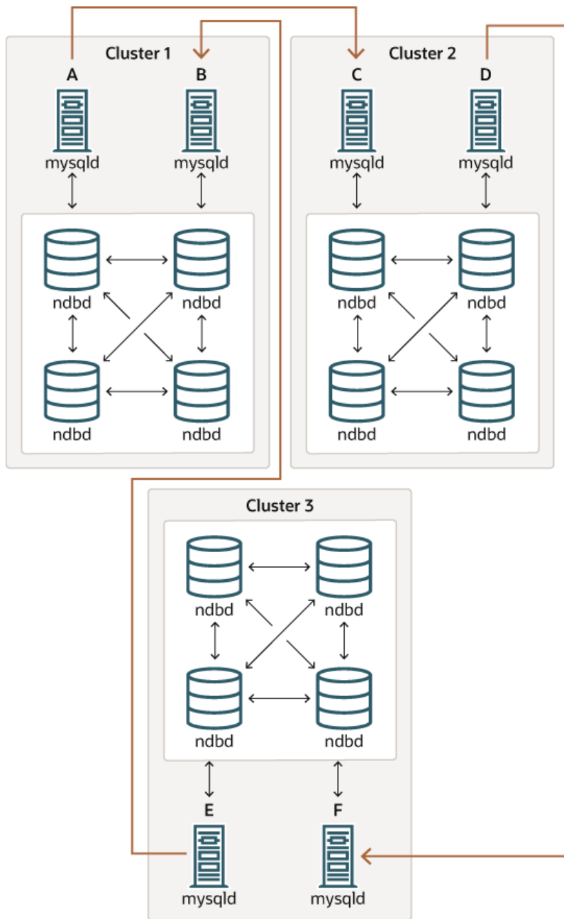
Figure 23.16 NDB Cluster Circular Replication Where Not All Sources Are Replicas
