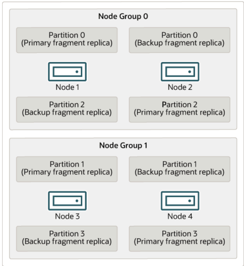
Figure 23.2 NDB Cluster with Two Node Groups
