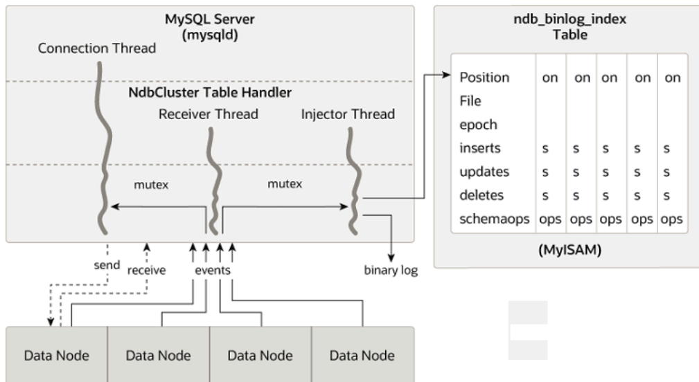
Figure 23.14 The Replication Source Cluster
