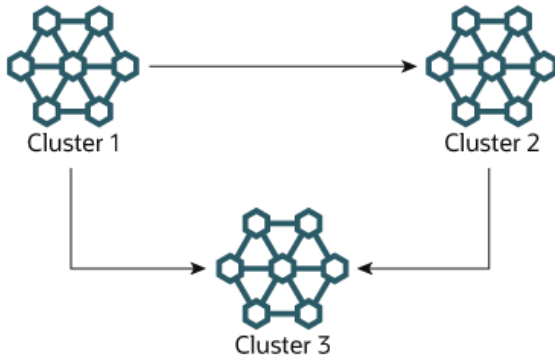
Figure 23.17 NDB Cluster Multi-Master Replication With 3 Sources
