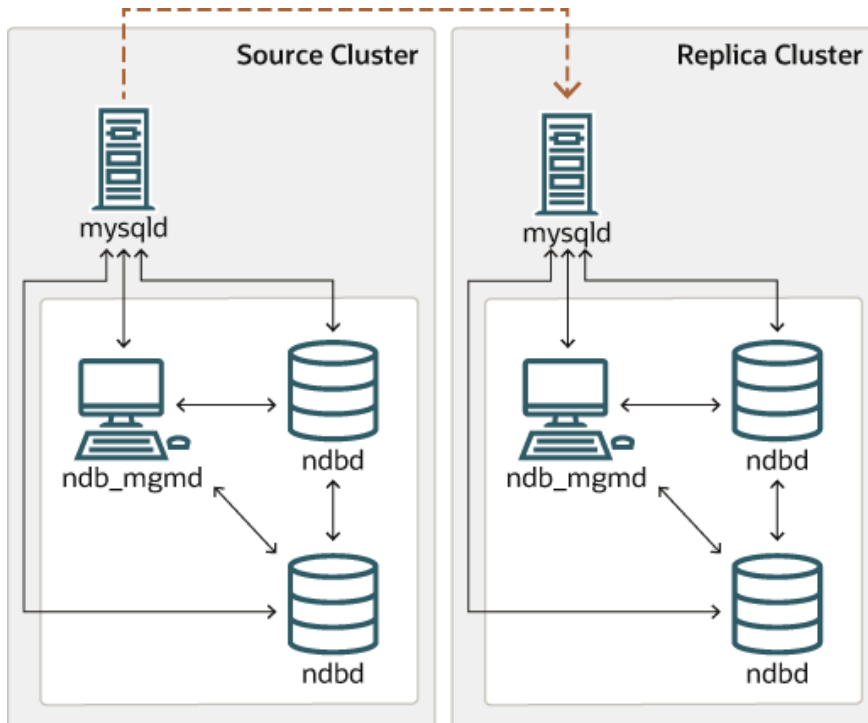
Figure 23.13 Replication Between SQL Nodes Connected Using IPv6
