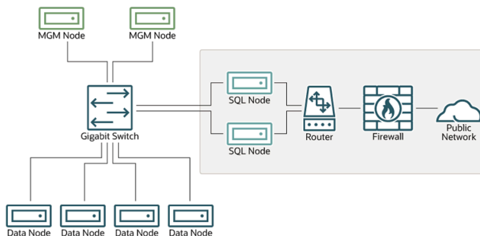
Figure 23.7 NDB Cluster with Hardware Firewall
