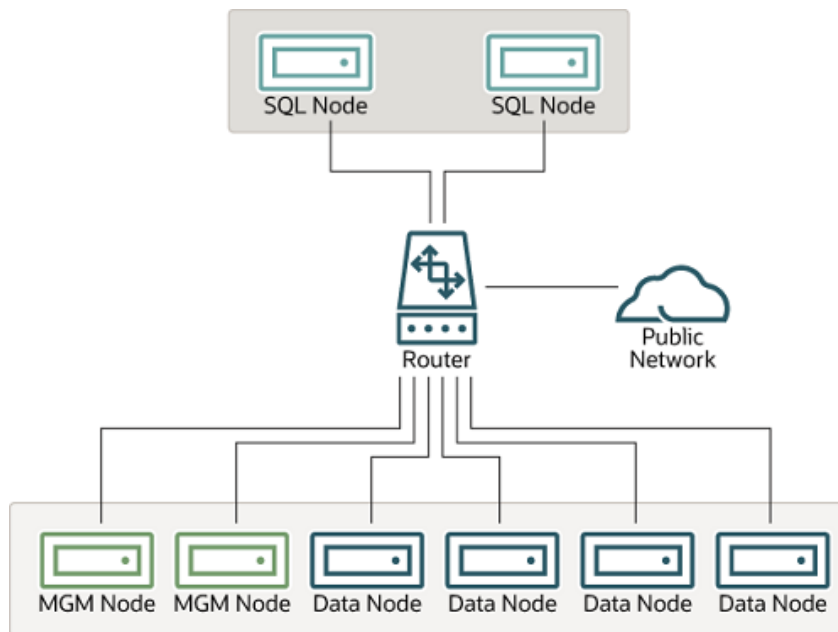
Figure 23.8 NDB Cluster with Software Firewalls
