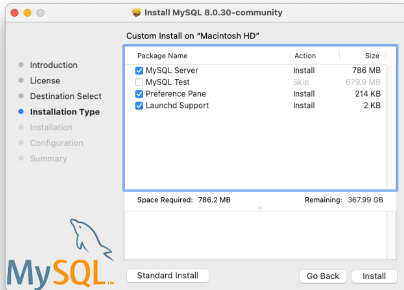
Figure 2.14 MySQL Package Installer Wizard: Customize
