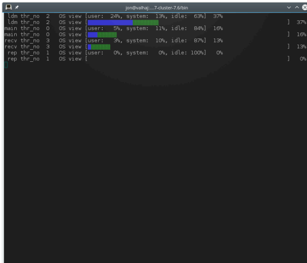
Figure 23.5 ndb_top Running in Terminal
