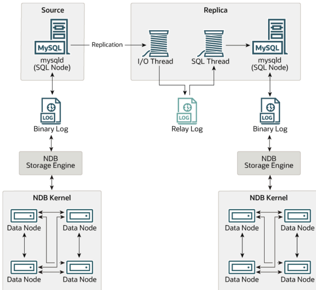
Figure 23.10 NDB Cluster-to-Cluster Replication Layout
