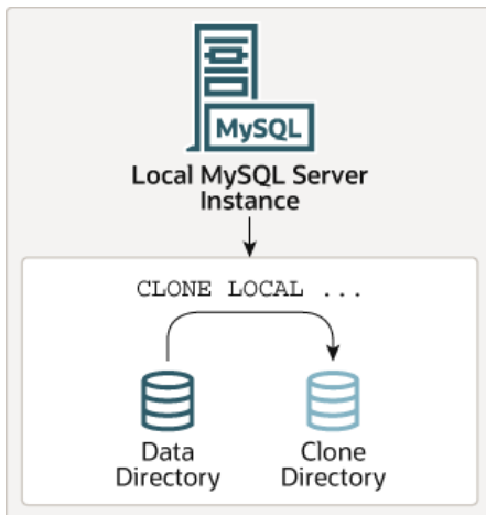
Figure 5.1 Local Cloning Operation
