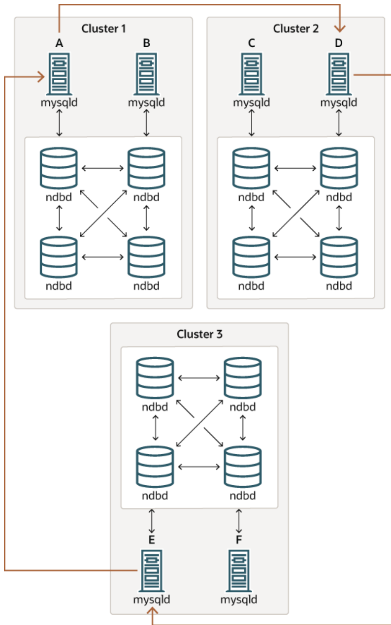
Figure 23.15 NDB Cluster Circular Replication with All Sources As Replicas
