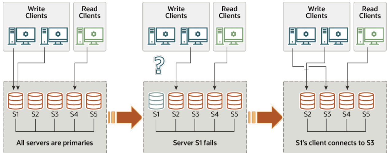
Figure 18.5 Client Failover
