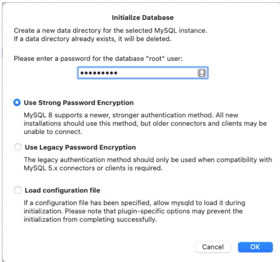
Figure 2.23 MySQL Preference Pane: Initialize Database
