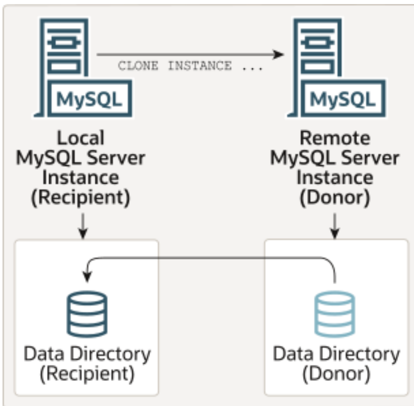
Figure 5.2 Remote Cloning Operation
