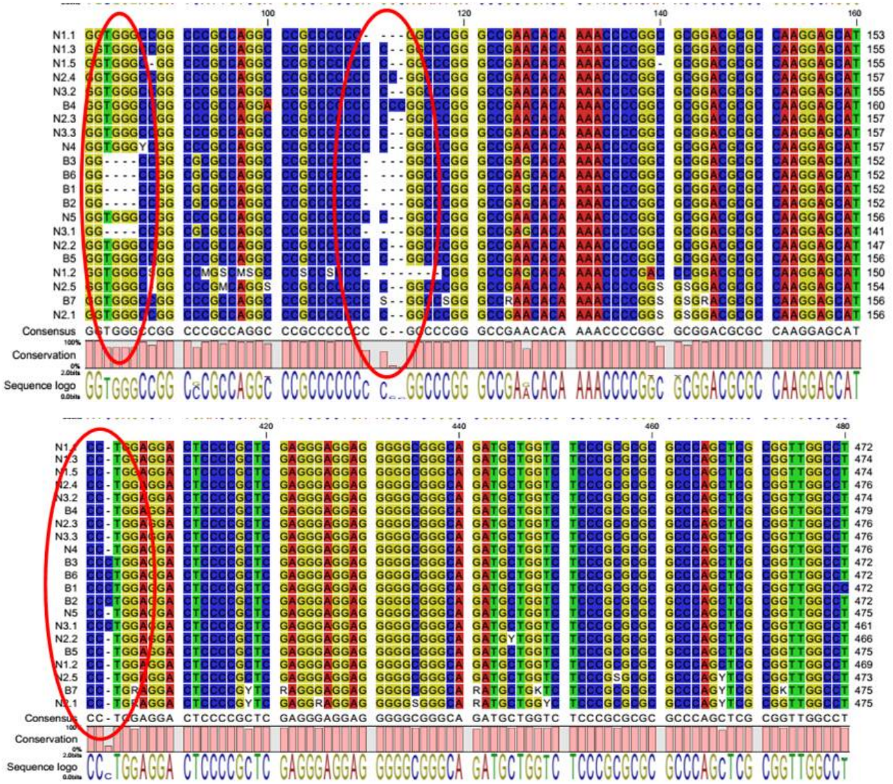
Figure 3. Aligned sequence of ITS regions of the Ochna samples.
