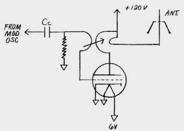
CARRIER OSCILLATOR
