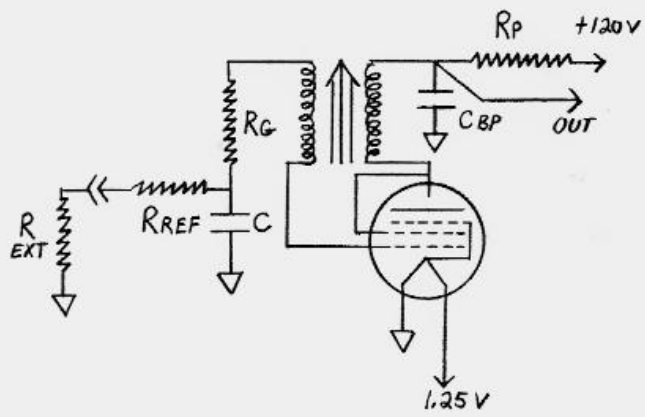
MODULATION OSCILLATOR
