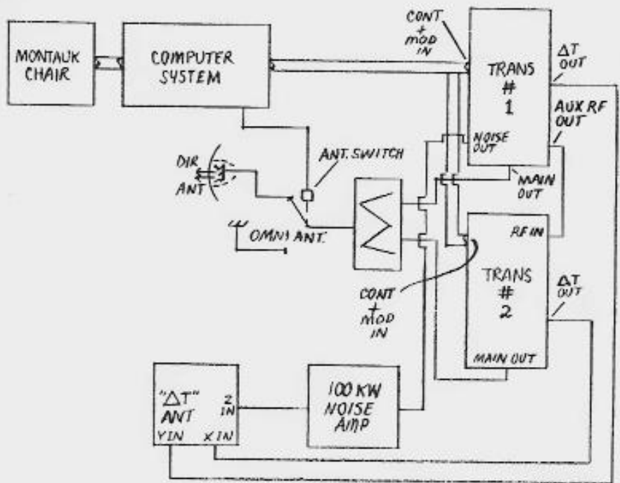
OVERALL BLOCK DIAGRAM
