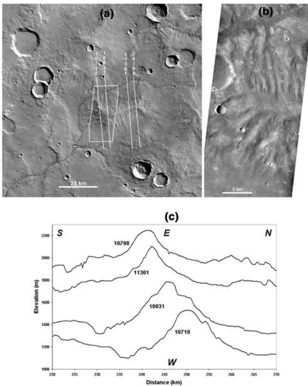
Figure 14. A gullied hill located at about -31.5^\circ lat., 9^\circ long. provides additional evidence for rainfall and surface runoff. (A) Context picture showing location of (B) and MOLA tracks in (C). Images from Viking Orbiter F084A. Regional valley network shown in black dashed lines. (B) MOC image AB107706 with an original resolution of about 15 m/pixel. (C) Selected MOLA profiles crossing the gullied hill, identified by orbit number. Distance scale is arbitrary. Profile 10031 is displaced vertically by +200 m, 11301 by +600 m, and 10798 by +700 m. Vertical exaggeration is about 28X.
