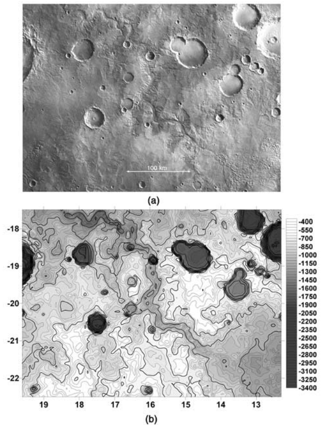
Figure 3. The relationship between fluvial dissection and topography in the vicinity of Loire Valles. (A) Regional mosaic of Viking images from orbit F615A centered at about -20^\circ lat., 15^\circ long. (B) Topography of the same region based upon MOLA data released through 30 August 1999. The contour interval is 100 m and the scale is in kilometers.
