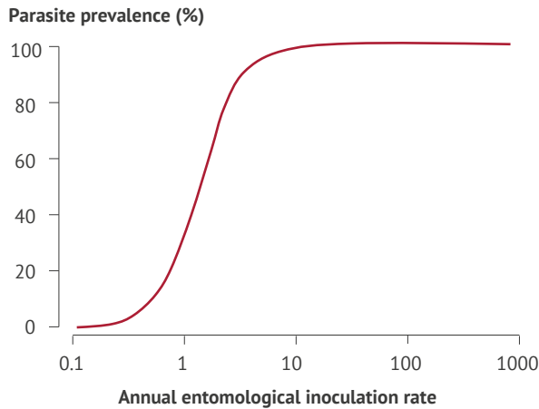
Figure A2.1. Relation between entomological inoculation rate and parasite prevalence (on the assumption that no infections are treated)
