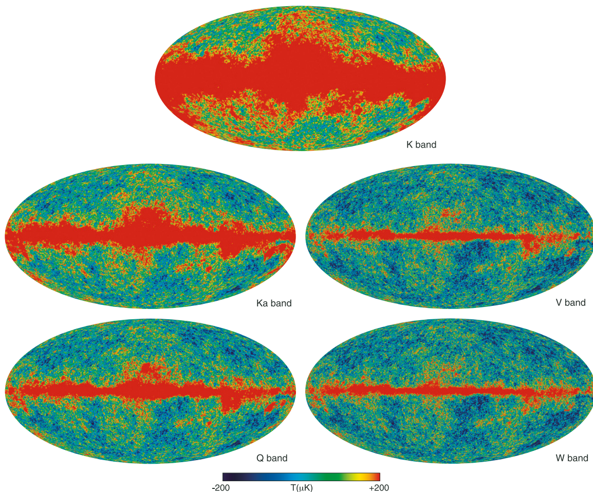
Figure 1. Five-year temperature sky maps in Galactic coordinates smoothed with a 0.2 Gaussian beam, shown in Mollweide projection. Top: K band (23 GHz), middle-left: Ka band (33 GHz), bottom-left: Q band (41 GHz), middle-right: V band (61 GHz), and bottom-right: W band (94 GHz).
