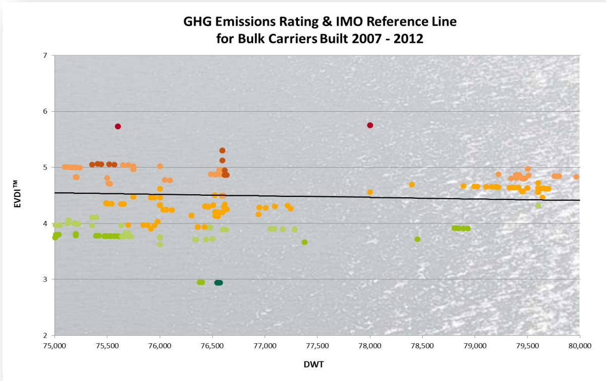
Figure 11: GHG Emissions Rating & IMO Reference Line for Bulk Carriers Built 2007 – 2012
