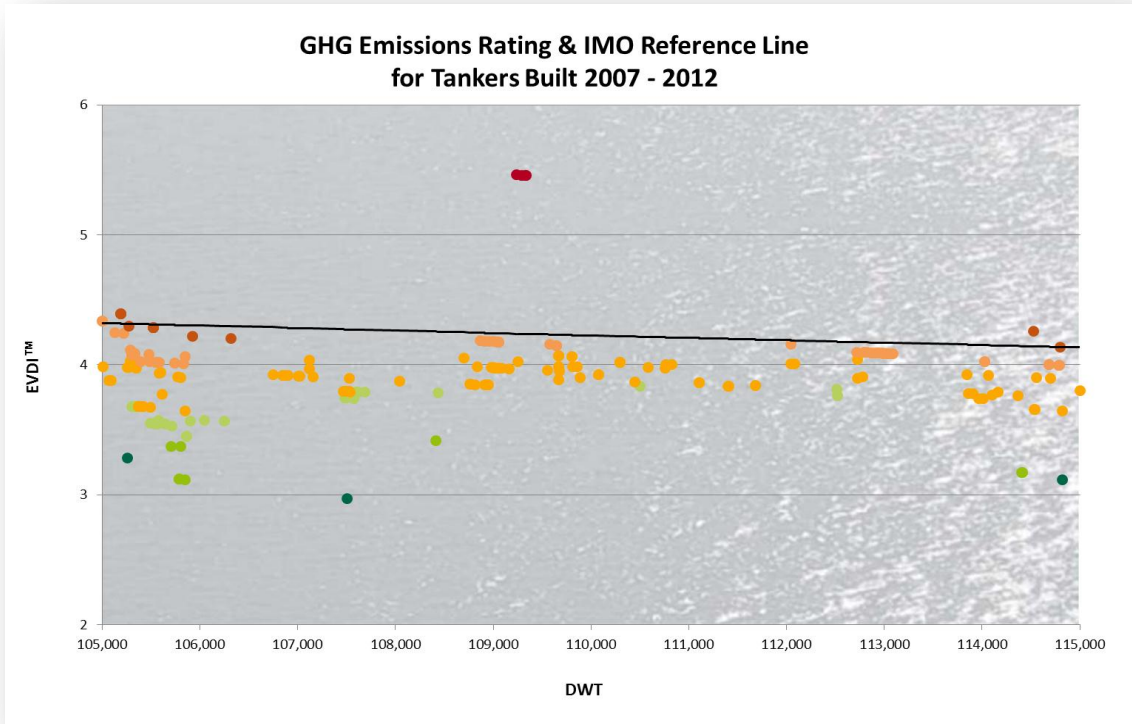
Figure 12: GHG Emissions Rating & IMO Reference Line for Tankers Built 2007 – 2012
