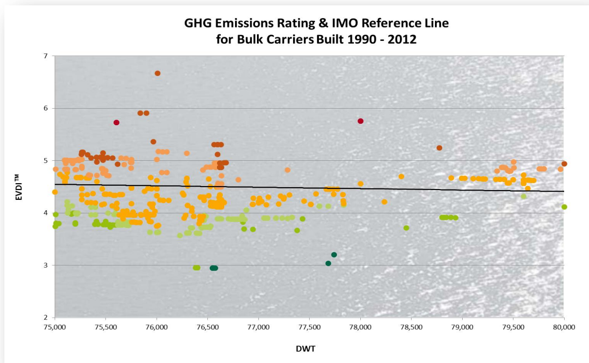
Figure 10: GHG Emissions Rating & IMO Reference Line for Bulk Carriers Built 1990 – 2012
