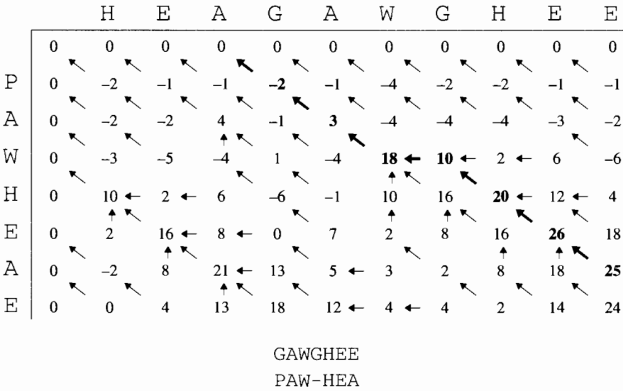
Figure 2.8 Above, the overlap dynamic programming matrix for the example sequences. Below, the optimal overlap alignment, with score 25.
