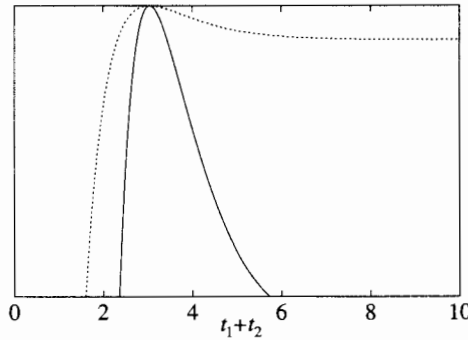
Figure 8.3 The log likelihood P(x^1, x^2|T, t_1, t_2) given by (8.9), with n_1 = 100, n_2 = 250 , and with n_1 = 1000, n_2 = 2500 . The latter curve is sharper, as there are more data to define the maximum likelihood peak. The curves have been shifted so their peaks superimpose.
