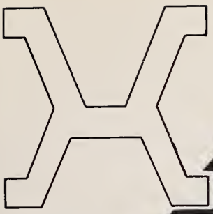
Tresca cross section. (twice size)
