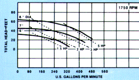
PV 4 x 4 x 10B
