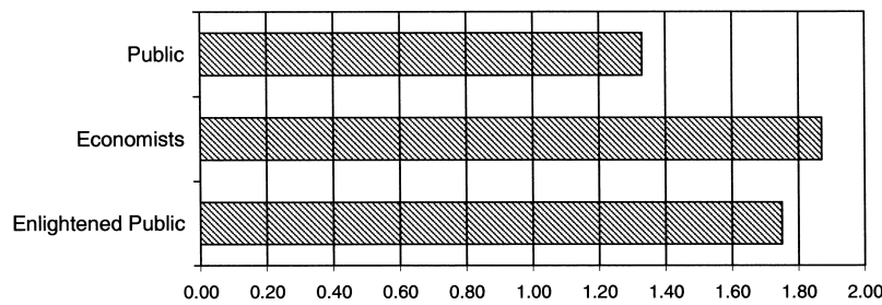
Figure 3.22 Question 22: "Trade agreements between the United States and other countries" 0 = "bad" 1 = "doesn't make much difference" 2 = "good"
