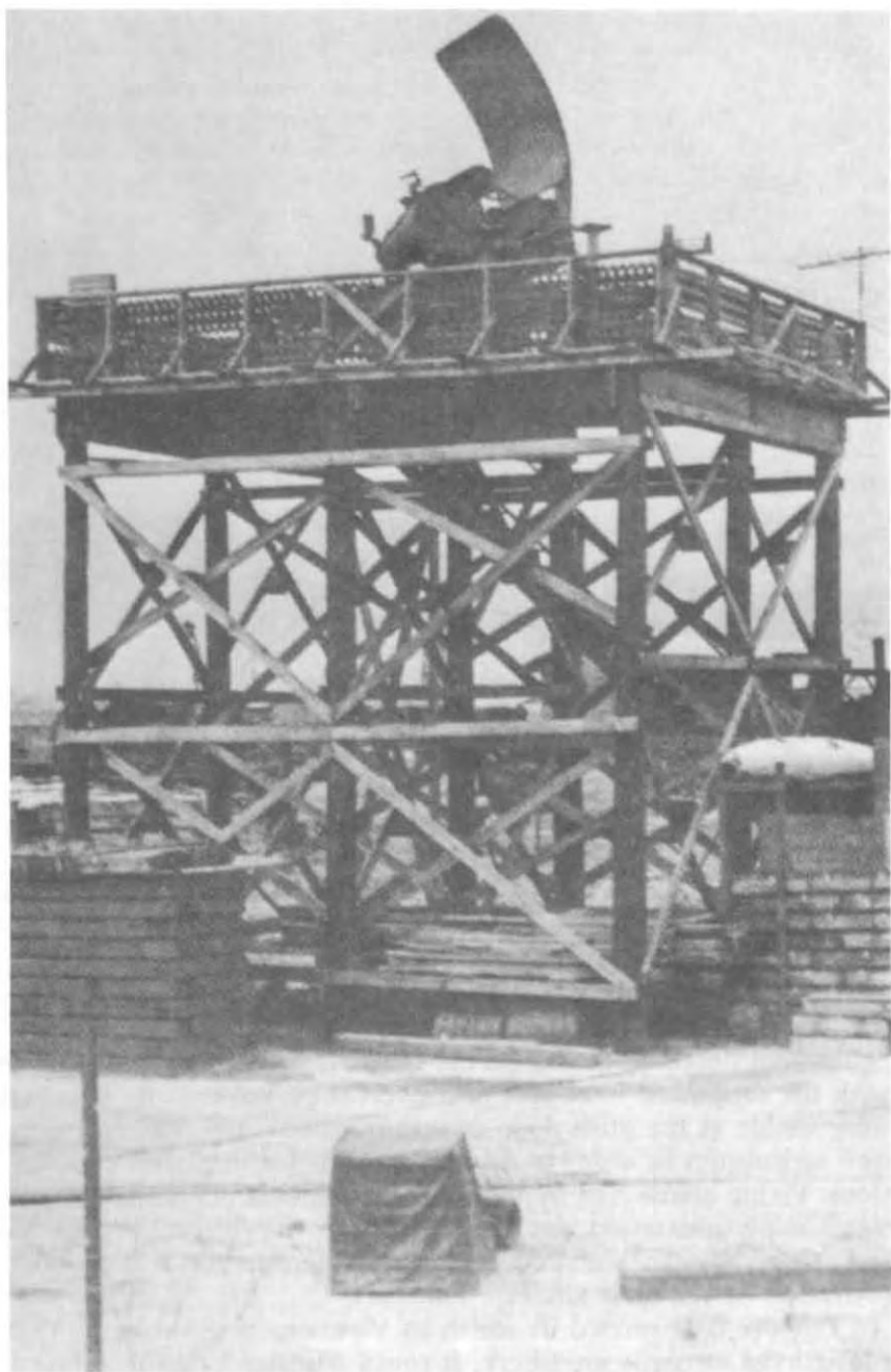
AN/MPQ-4 COUNTERMORTAR RADAR, positioned on a large tower for better area coverage.
