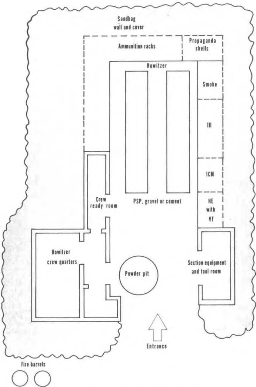
Diagram 3. Semipermanent 105-mm. self-propelled howitzer emplacement.
