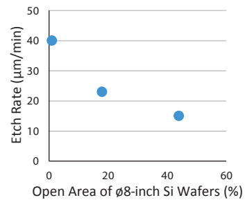
Fig. 2 Open Area of ø8-inch Si Wafers vs. Etch Rate
