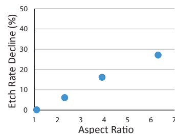
Fig. 3 Aspect Ratio vs. Etch Rate Decline
