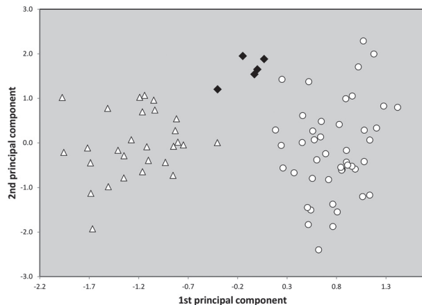
Fig. 28: Principal component analysis separating 45 gynes of the Normal morph (white circles), 28 gynes of the Rubens morph (white triangles) and 5 gynes of the Beishan morph (black rhombs) of Formica exsecta . Fifteen morphological characters were considered.
