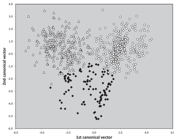
Fig. 27: Linear discriminant analysis separating 345 workers of the Normal morph (white circles), 253 workers of the Rubens morph (white triangles) and 110 workers of the Beishan morph (black rhombs) of Formica exsecta . Eight morphological characters were considered. The structuring within the clusters of the Normal and Beishan morphs is an artefact caused by the discrete 1-2-3-4-5 data format of ClySet.
