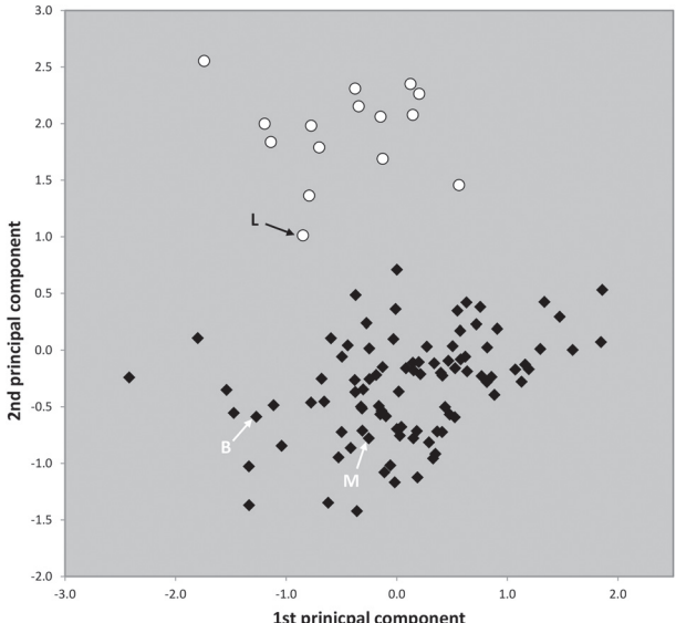
Fig. 32: Nest sample means of the 1 st and 2 nd principal components of 94 nest samples of Formica manchu (black rhombs) and 15 nest samples of F. longiceps workers (white discs). Twelve phenotypic characters were considered. Arrows point to the type series of F. longiceps (L), F. manchu (M) and F. beijingensis (B).
