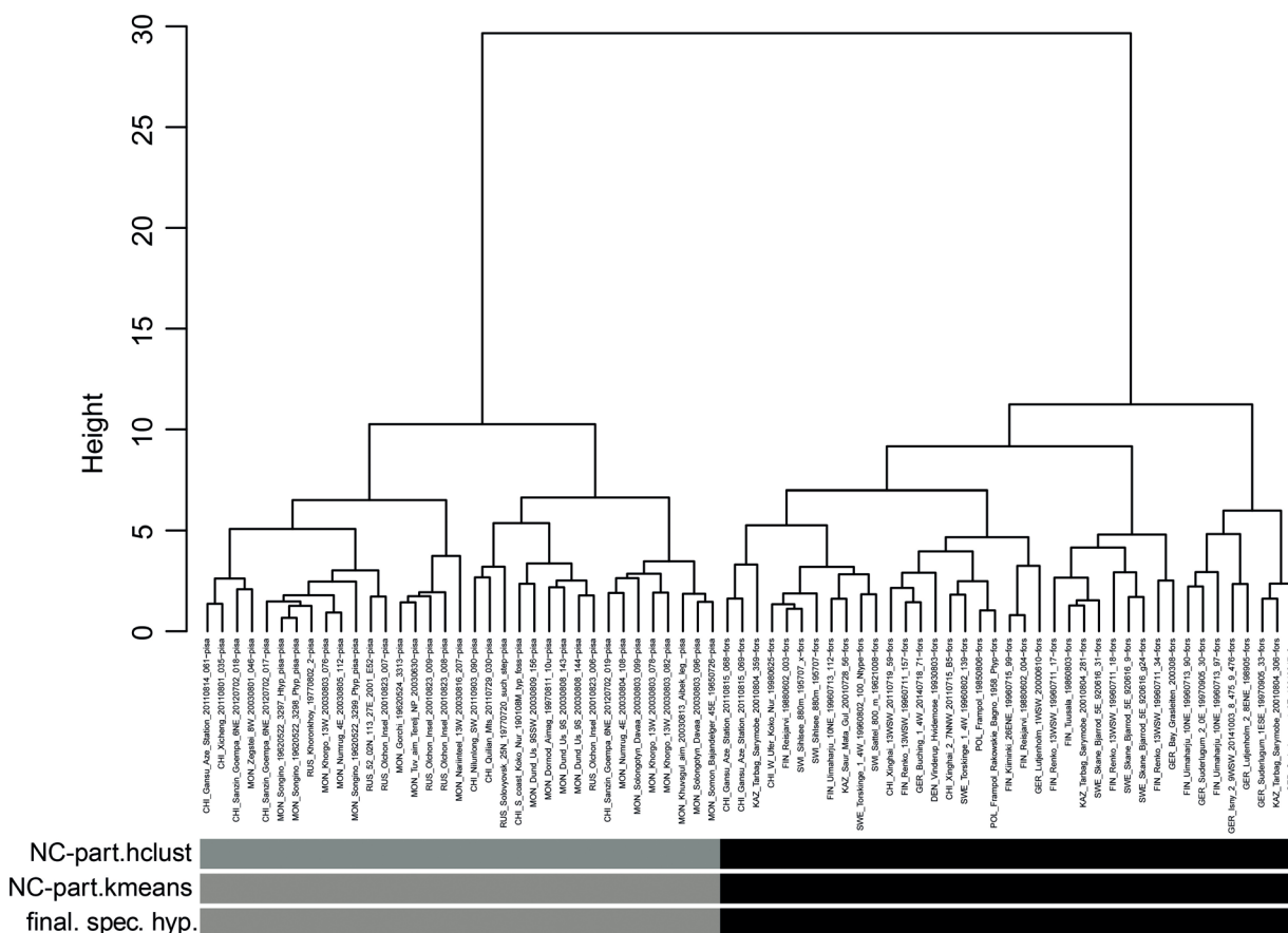
Fig. 40: Classification by NC-Ward clustering (dendrogram shown), NC-part.hclust clustering and NC-part.kmeans clustering of 74 worker nest samples of Formica forsslundi (black bars) and F. pisarskii (grey bars) considering six morphological characters. The mean error of the three exploratory analyses relative to the controlling LDA is 0 %.
