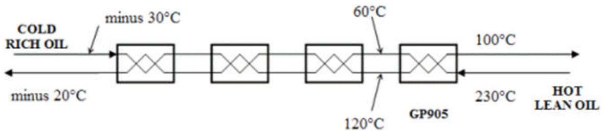
Fig. 1 – Extremely simplified schematic arrangement of GP905 & other exchangers (temperatures are nominal only, for normal operations)
