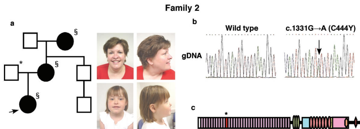
Figure 2. NOTCH2 mutation in family 2. a , Proband, her mother, and her grandmother had clinical features associated with AGS. The family member marked with an asterisk (*) was tested for the presence of the mutation but had only wild-type sequence. Individuals marked with a section symbol (§) had mutant sequences. b , Sequence analysis shows a mutation in exon 8 in all three affected individuals. c , The mutation (asterisk) is predicted to cause substitution of a tyrosine for a cysteine residue in EGF-like repeat 11 of Notch2.
