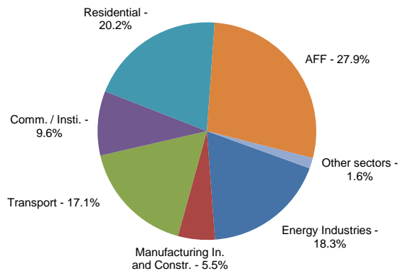
Figure 16.2.4 CO 2 emissions, distribution according to the main sectors for 2020.
