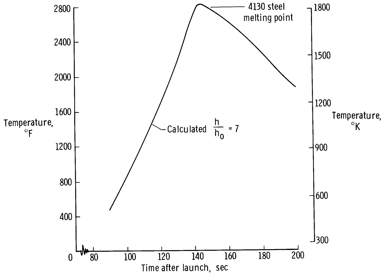
Figure 13. - Calculated temperature time history of cowl-lip interference zone.
