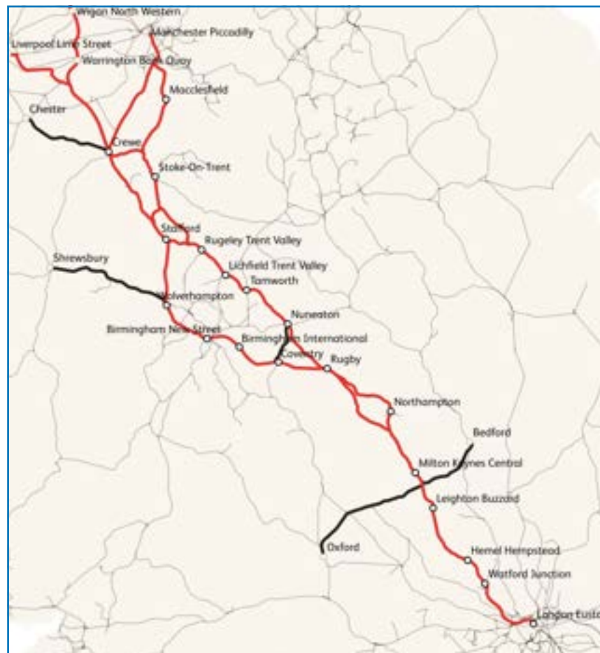
Figure 6: West Coast South electrification map, including primary interfacing routes over which future passenger services identified in this report could run.
