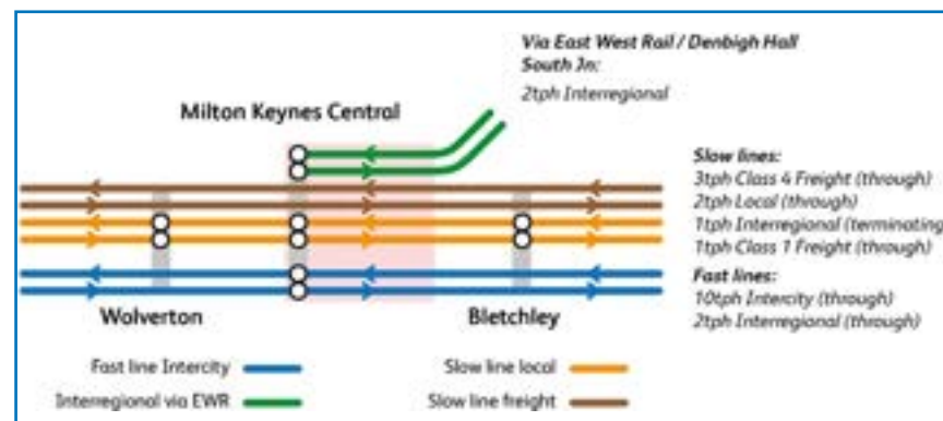
Figure 37: Capacity bottleneck Bletchley-Milton Keynes in the Intermediate Markets released capacity train plan.
