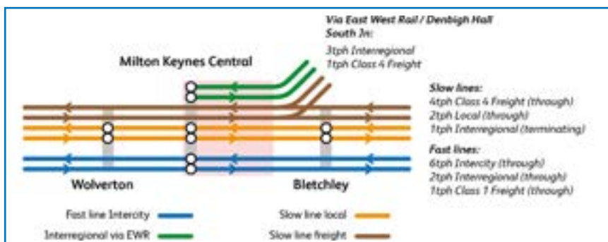
Figure 32: Capacity bottleneck Bletchley-Milton Keynes in the freight scenario released capacity train plan
