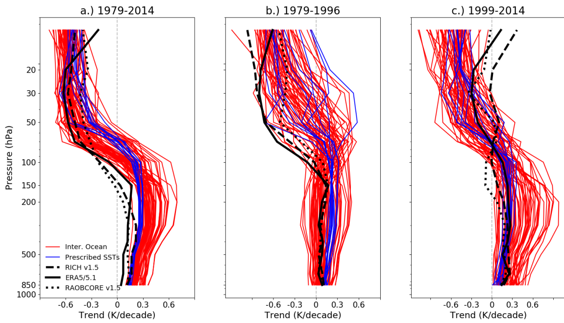
Figure S3. As in Figure ??a but with different trend averaging periods for panel b and c.
