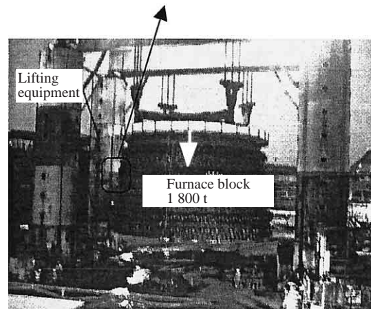
Photo 2 4 points supporting in lifting equipment
