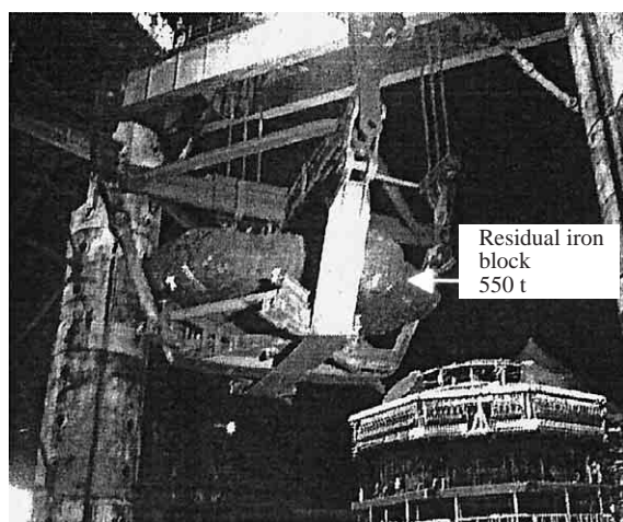
Photo 3 Hanging up large residual iron block
