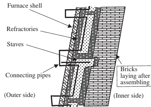
Fig. 5 The section of furnace block
