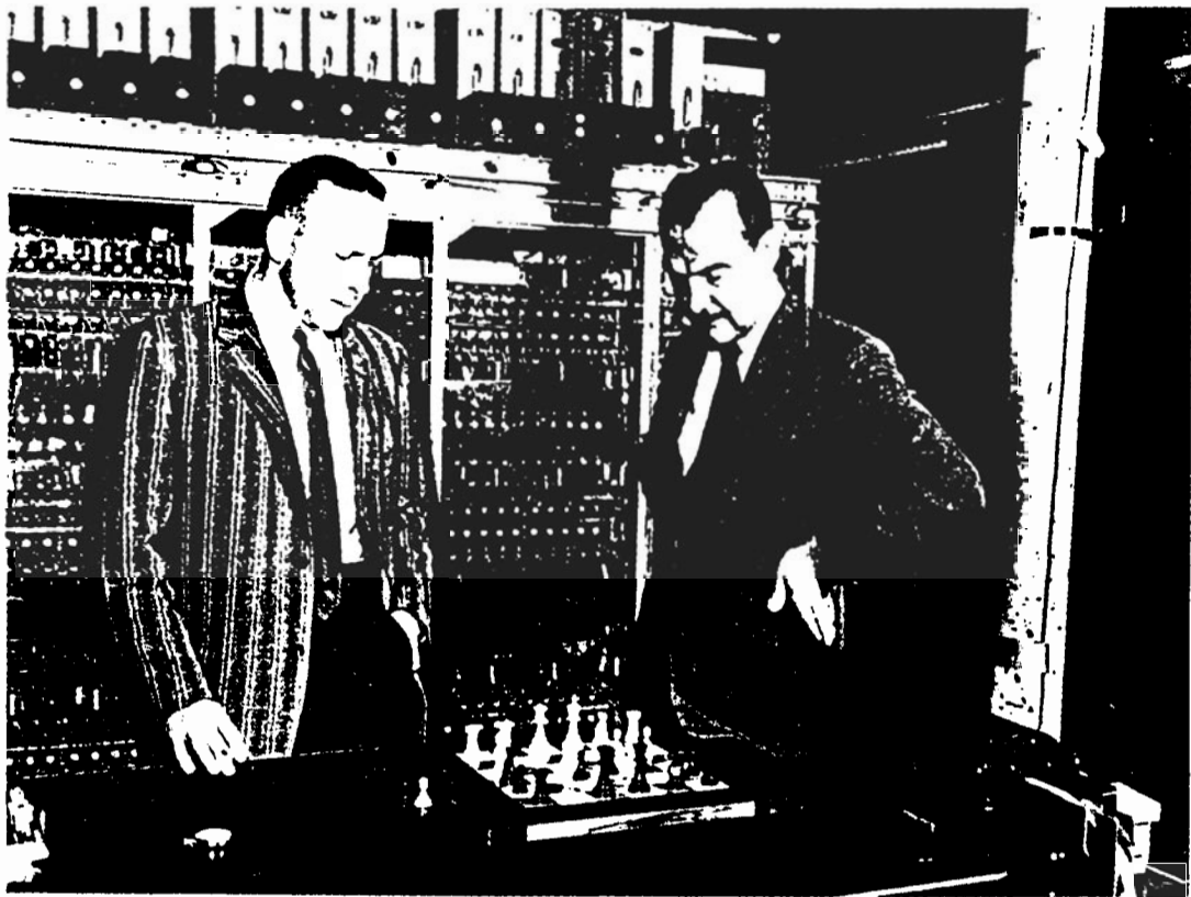
Fig. 7. Paul Stein and Nick Metropolis at the MANIAC and the 6×6 anticlerical chess board.
