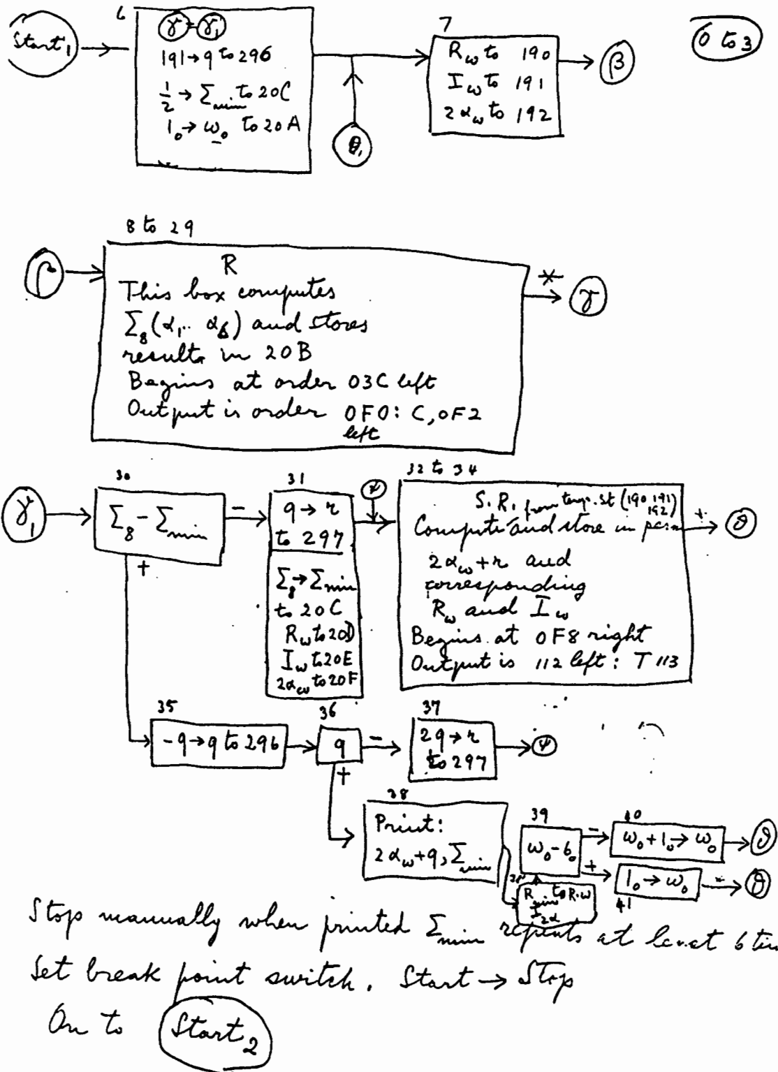
Fig. 4. Fermi's program for the MANIAC: calculation of the phase shifts.
