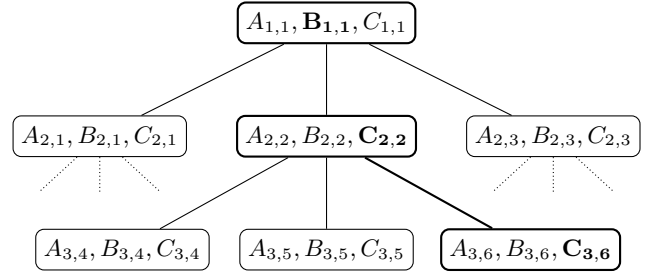
Figure 1: A tree as in our construction
