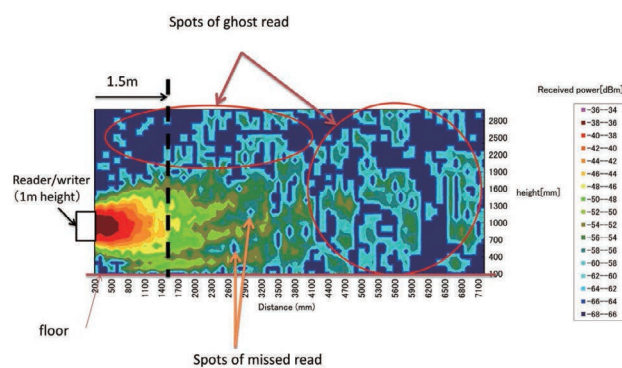
Received power map
